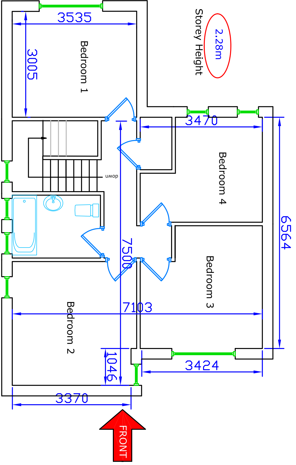
VEPC 1 FIRST FLOOR PLAN
